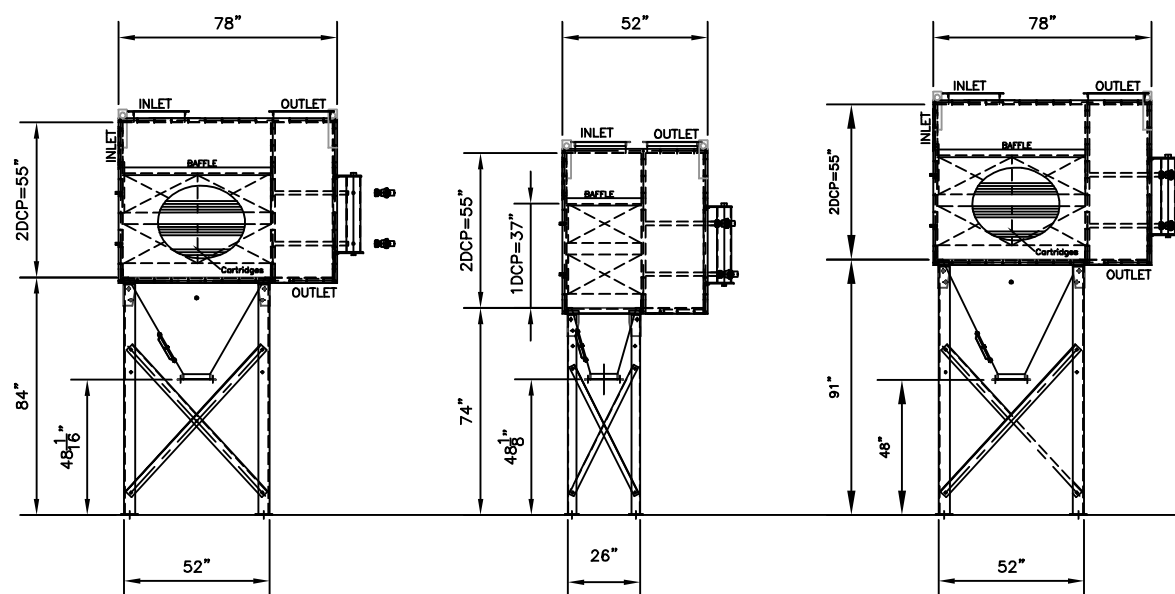
SIDE ELEVATION 2DCP-8 & 24
