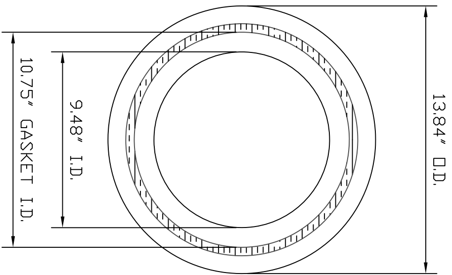
OPEN TOP WITH GASKET
